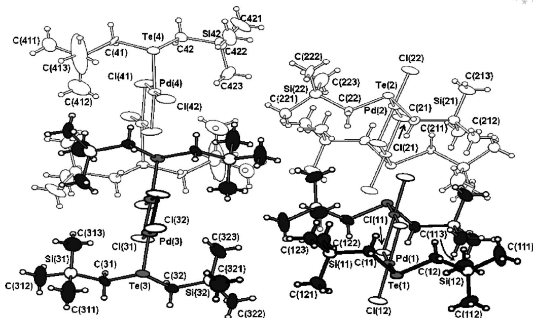
Figure 4. Molecular structure of [\text{Pd}_2(\mu\text{-Cl})_2\text{Cl}_2\{\text{Te}(\text{CH}_2\text{SiMe}_3)_2\}_2] ( 5 ) indicating the numbering of atoms. The thermal ellipsoids have been drawn at 50% probability level.
