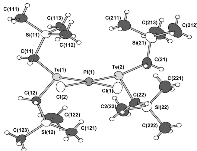
Figure 1. Molecular structure of cis - [\text{PtCl}_2\{\text{Te}(\text{CH}_2\text{SiMe}_3)_2\}_2] ( 2c ) indicating the numbering of atoms. The thermal ellipsoids have been drawn at 50% probability level.
