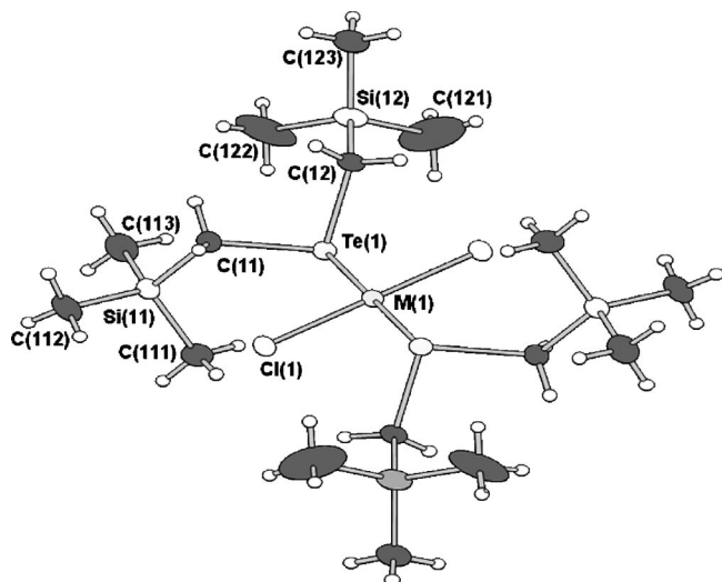
Figure 2. Molecular structure of trans\text{-}[MCl_2\{\text{Te}(\text{CH}_2\text{SiMe}_3)_2\}_2] [ M = \text{Pt} ( 2t ), \text{Pd} ( 3t )] indicating the numbering of atoms. The thermal ellipsoids have been drawn at 50% probability level.
