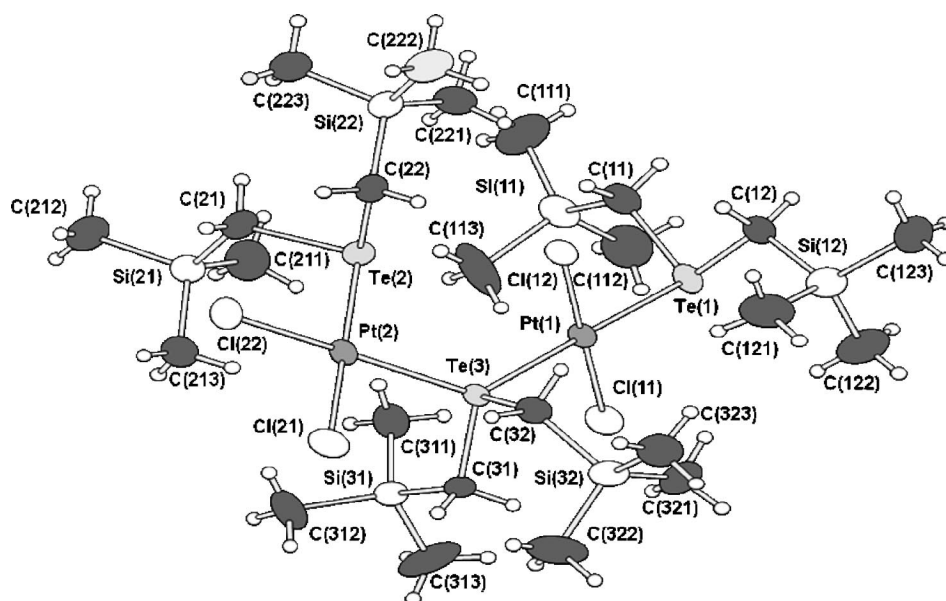
Figure 3. Molecular structure of [\text{Pt}_2\text{Cl}_4\{\mu\text{-Te}(\text{CH}_2\text{SiMe}_3)_2\}\{\text{Te}(\text{CH}_2\text{SiMe}_3)_2\}_2] ( 4 ) indicating the numbering of atoms. The thermal ellipsoids have been drawn at 50% probability level.
